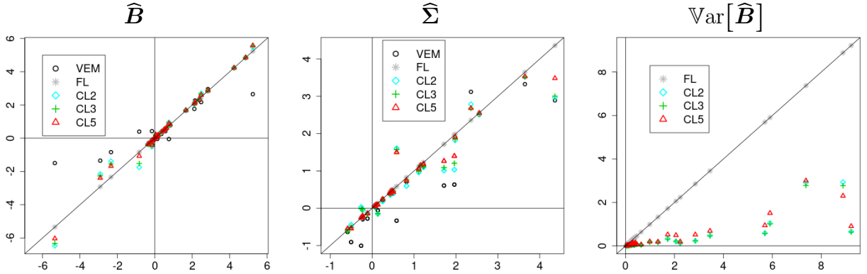
Figure 6: Comparison of the estimates with the different algorithms for the Barents sea reduced data set ( p = 7 species). Left: regression coefficients \widehat{\beta}_{hj} , center: covariance parameters \widehat{\Sigma}_{jk} , right: estimated variances of the regression coefficients \widehat{\beta}_{hj} . x -axis = full likelihood inference (FL), y -axis: likelihood inference (FL = gray asterisk [*] = reference), composite likelihood inference (CL2 = cyan diamond [ \diamond ], CL3 = green plus sign [+], CL5 = red triangle [ \triangle ]) and variational EM (VEM = black circles [ \circ ]).
