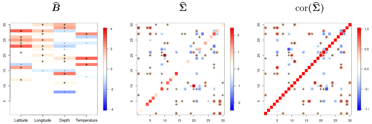
Figure 9: Colormap of the parameter estimates the Barents sea full data set ( p = 30 species). Left: regression coefficients \widehat{\beta}_{\ell j} , center: covariance parameters \widehat{\Sigma}_{jk} , right: corresponding correlations \widehat{\rho}_{jk} = \widehat{\Sigma}_{jk} / \sqrt{\widehat{\Sigma}_{jj}\widehat{\Sigma}_{kk}} . Blank cells correspond to non-significant estimates, red cells (marked with '+') to positive estimates and blue cells (marked with '-') to negative estimates.
