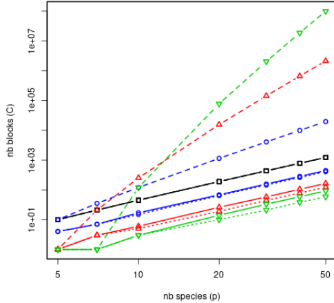
Figure 1: Number of blocks C as a function of the number of species p (in log-log-scale) for blocks of size k = 2 (black squares \blacksquare ), k = 3 (blue circles \circ ), k = 5 (red triangles up \triangle ) and k = 7 (green triangles down \nabla ). Solid line: number of blocks actually used, dashed line: upper bound \binom{p}{k} , dotted line: lower bound p(p-1)/[k(k-1)] .
