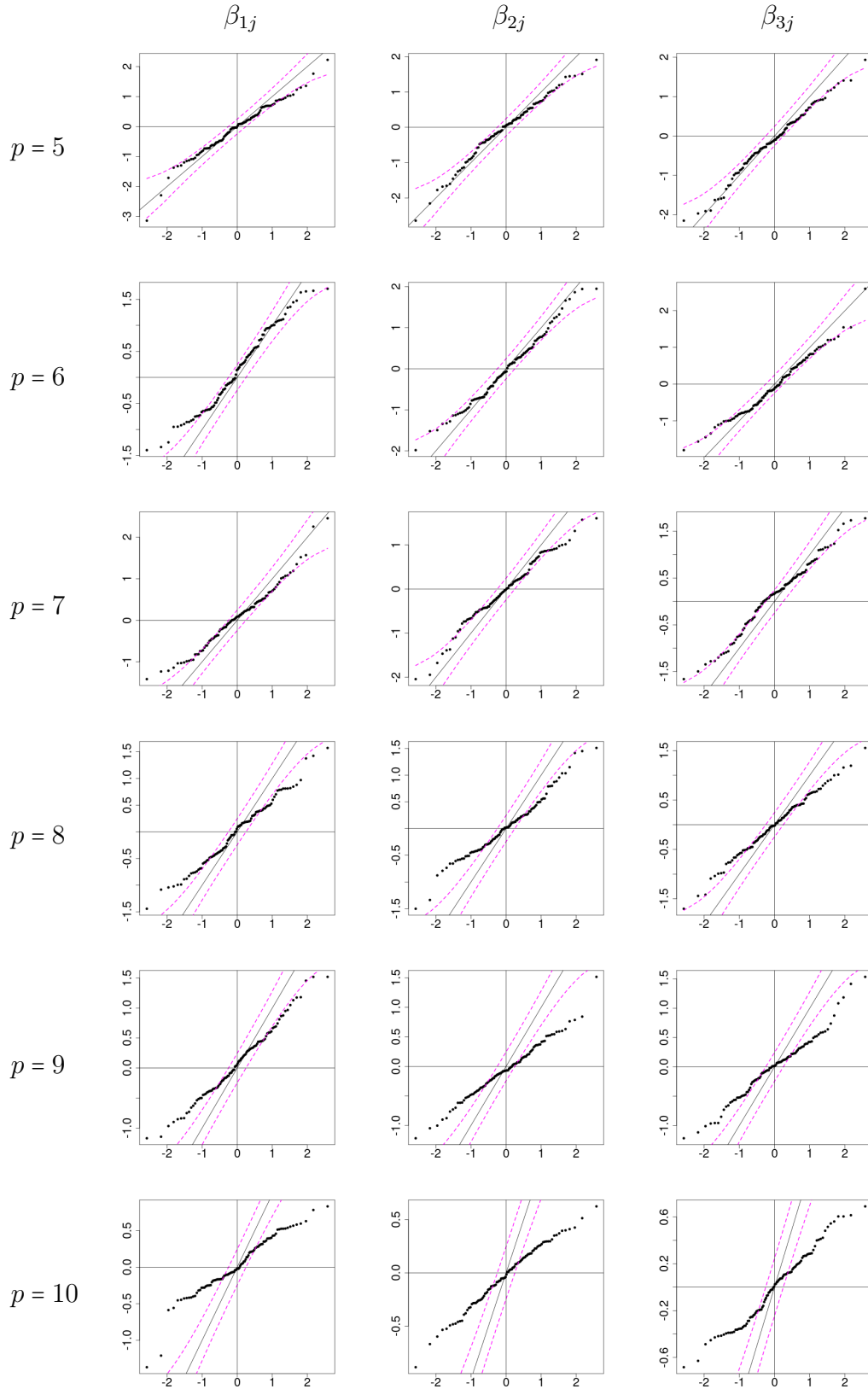
Figure 11: qq-plots of the normalized regression coefficient \tilde{\beta}_{ej} defined in Equation (22) for the second simulated species for each of the d = 3 covariates with full likelihood (FL) with p = 5, \dots, 10 species. Same legend as Figure 3.
