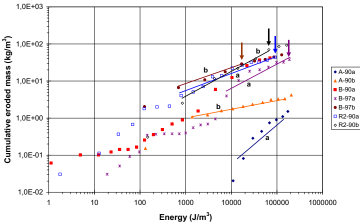
Figure 5. Cumulative eroded dry mass in terms of the cumulative energy expanded by the water to seep through the soil.
