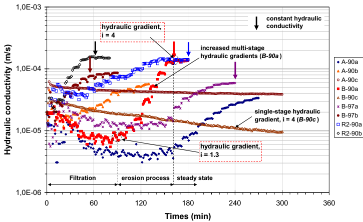
Figure 3. Time series of hydraulic conductivity
