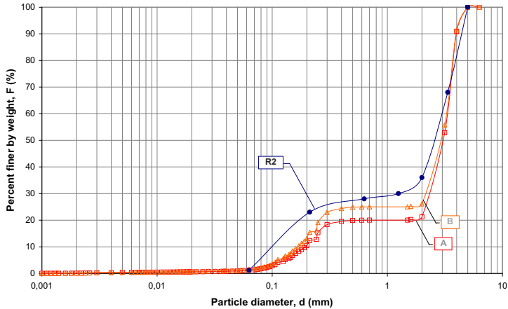
Figure 1. The particle size distribution of tested specimens
