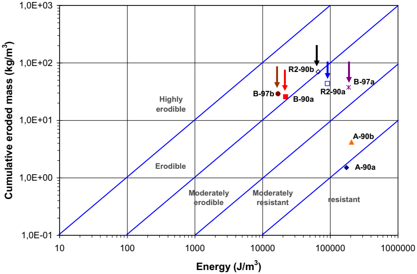
Figure 6. Classification of suffusion sensibility based on the energy expended by the water seepage in the soil
