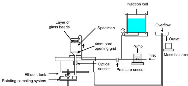
Figure 2. Schematic diagram of the erodimeter
