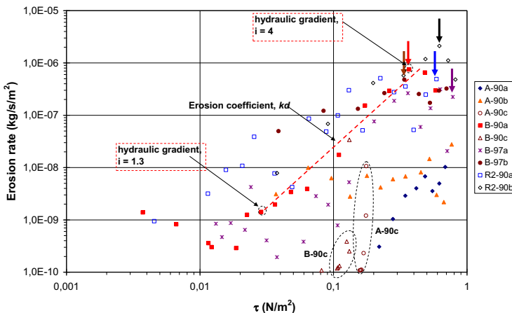
Figure 4. Erosion rate versus hydraulic shear stress
