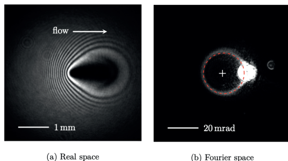
Figure 1. Scattering of the fluid on an attractive or repulsive defect. a) Density distribution (real space imaging). b) Momentum space distribution (Fourier space imaging)
