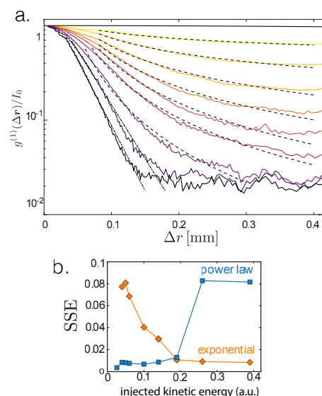
Figure 2. Emergence of an out-of-equilibrium BKT transition in optics. First order correlation function with increasing fluctuation strength \epsilon , transition from an algebraic to an exponential order. quenches.
