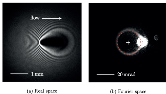
Figure 1. Scattering of the fluid on an attractive or repulsive defect. a) Density distribution (real space imaging). b) Momentum space distribution (Fourier space imaging)
