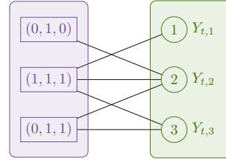
Figure 1: Stochastic combinatorial semi-bandit setting where d = 3 , \mathcal{A} = \{(0, 1, 0), (1, 1, 1), (0, 1, 1)\} , and P = |\mathcal{A}| = 3 .
