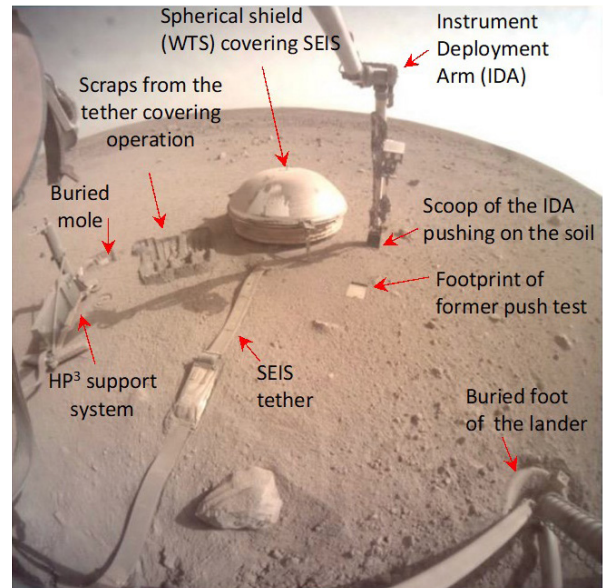
Figure 5. Image taken by the Instrument Context Camera on sol 1170 showing the SEIS WTS (diameter 720 mm) with the Instrument Deployment Arm (IDA) vertically pushing on the soil at the right of the SEIS. As described in more details in Section 5.3.2, the IDA is performing the second elastic pushing experiment, resulting in a tilt monitored by SEIS. The rectangular imprint of the back of the scoop is from the indentation and first elastic experiment. All instruments are covered by a dust layer progressively brought by the Martian winds (image credit: NASA-JPL).
