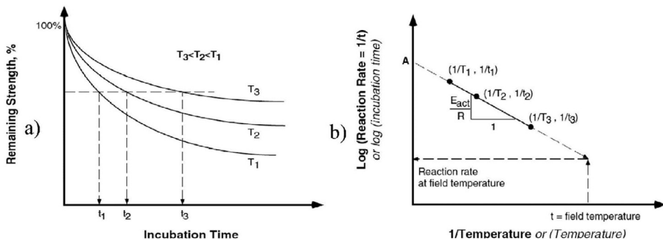
Fig. 1. Arrhenius plot [2].
