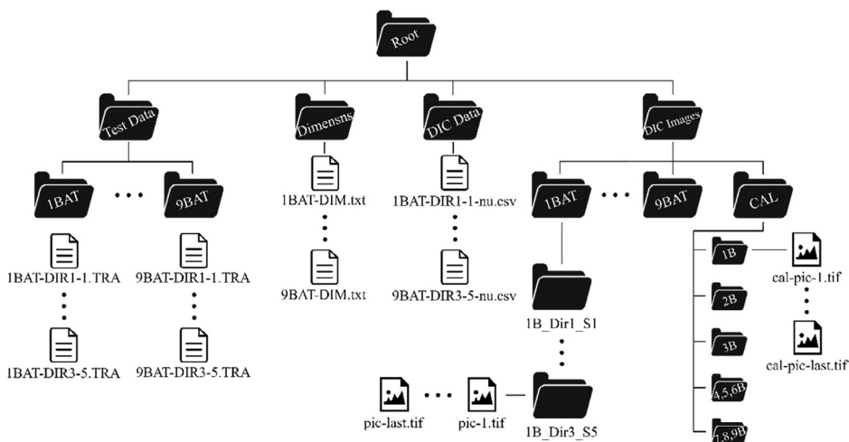
Fig. 2. Folder structure.
