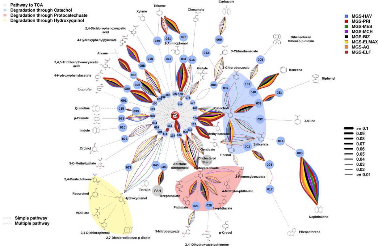
Figure 3. Potential aerobic and/or anaerobic degradation networks of alkanes and aromatics via di- and trihydroxylated intermediates in the investigated communities (see color code) after combining DNA- (Supplementary Fig. S2) and 16S rRNA-based (Supplementary Fig. S3) analyses. The biodegradation network reconstruction was performed as described in Supplementary Methods. Briefly, predicted open reading frames (ORFs) in the DNA or 16S rRNA-derived meta-sequences were filtered by score ( >45 ) and e-value ( <10e^{-3} ) according to their similarity to the sequences of key aromatic catabolic gene families involved in the degradation of aromatic pollutants and alkanes 24,27 . After a manual check, a final list of gene sequences encoding enzymes potentially involved in degradation was prepared. For network reconstruction, each sequence was assigned to a metabolic substrate and a product with an assigned code, and the putative substrates and products processed in the sample were connected, creating a metabolic network using appropriate scripts and commands (for details, see Supplementary Methods). The rel. ab. of each catabolic gene assigned to degradation reactions, as represented by the thickness of the lines in the figure, and the complete list of substrates possibly degraded by the communities are summarized in Supplementary Table S5. Confidence greater than 90% as indicated in Supplementary Table S5. Note that rel. ab. refers to the total number of genes in a given sample to avoid artifacts due to differences in sample size. The codes for the chemical species in each pathway are as described in Supplementary Fig. S2 and Table S5A.
