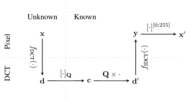
Fig. 3. JPEG pipeline illustrating the notations. The separation unknown/known refers to what the steganalyzer knows or does not.
