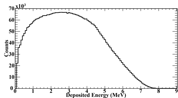
Figure 1. Measured \Delta E - E coincidences spectrum for the decay of ^{92}\text{Rb} .
