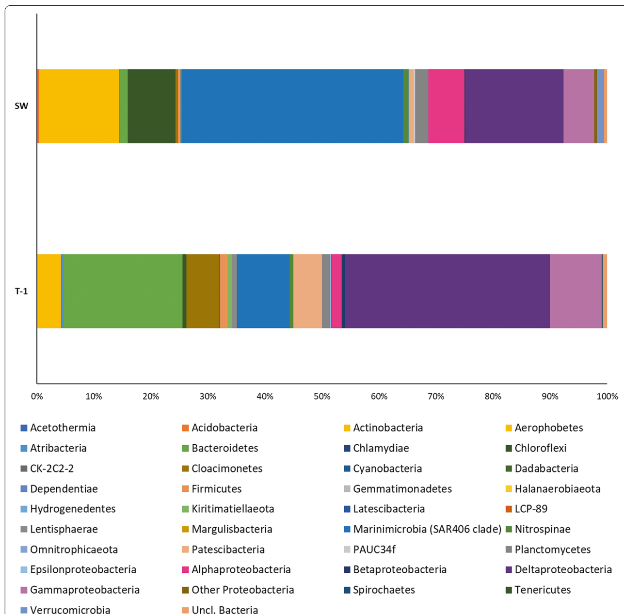
Fig. 2 Bacterial community composition in the Tyro upper seawater-brine interface (T-1) and overlying seawater (SW). The bar plots indicate the taxonomic composition (at the phylum level) of T-1 and SW bacterial communities. The composition of the Proteobacteria phylum in the samples is detailed at the class level
