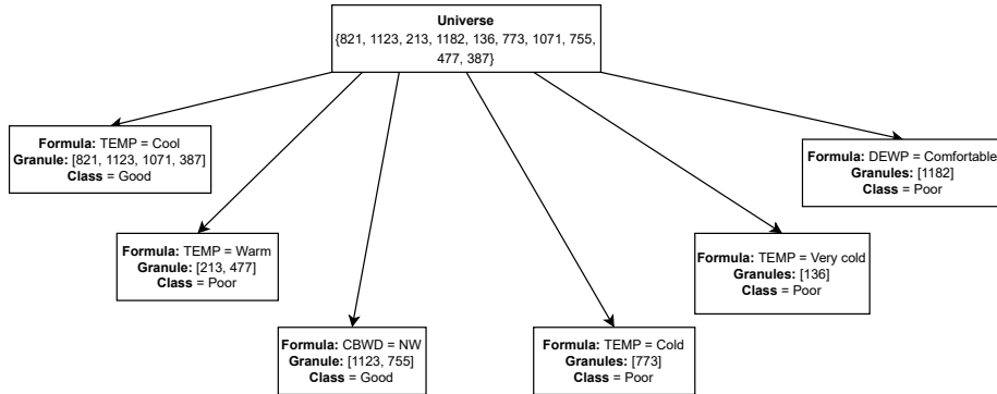
Figure 4: Granular tree demo
