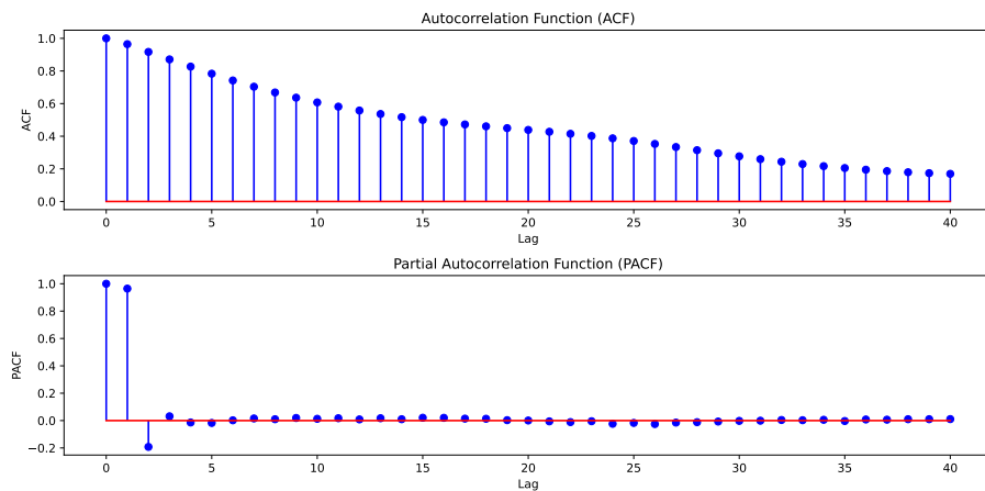
Figure 3: PM_{2.5} ACF and PACF plots
