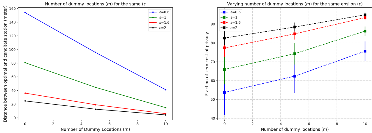
FIGURE 5: Impact of introducing dummy locations along with AGeoI on the CoP.
