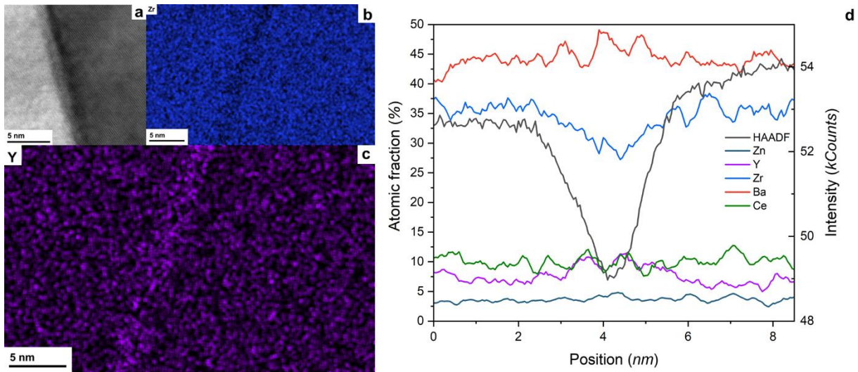
Figure 12 - (a) TEM image of a cross section of \text{BaZr}_{0.7}\text{Ce}_{0.2}\text{Y}_{0.1}\text{O}_{3-\delta} electrolyte fabricated using ZnO-Li, (b and c) EDX mapping of the ZnO-Li sample grain boundary {Zr and Y} and (d) evolution of the atomic distribution as a function of the map position on the sample
