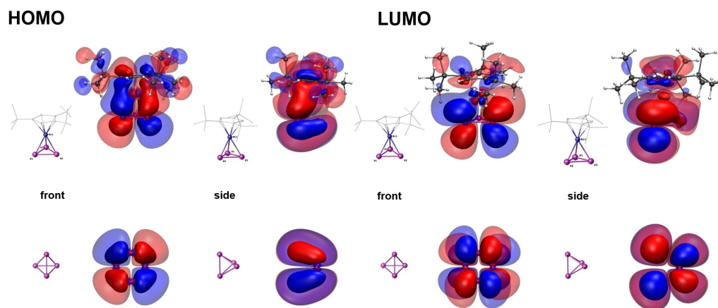
Figure 3. Frontier orbitals of the XRW (Mo K h ) model of [Ni]P 3 (upper half) compared to the DFT calculation of P 4 (lower half).
