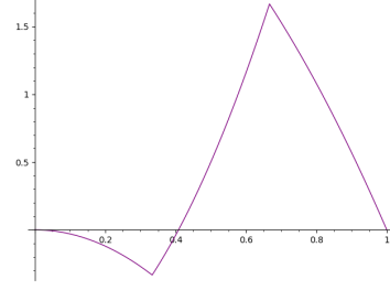
FIGURE 2. \kappa(t)
