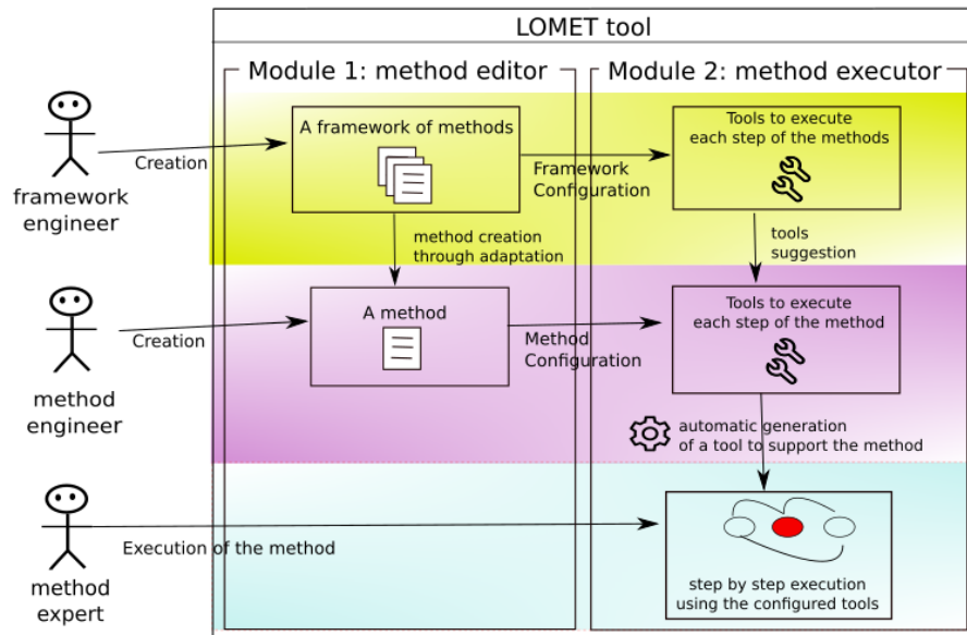
Fig. 1. A low-code approach to support Method Engineering.
