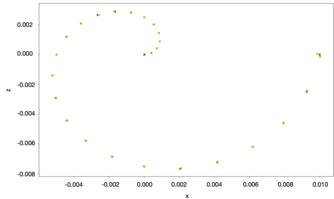
Fig. 6. Results obtained for the Liandford robot control for the first case: position on the x - z plane for the spiral trajectory. Green: the objective. Orange: position of the effector on the considering plane.
