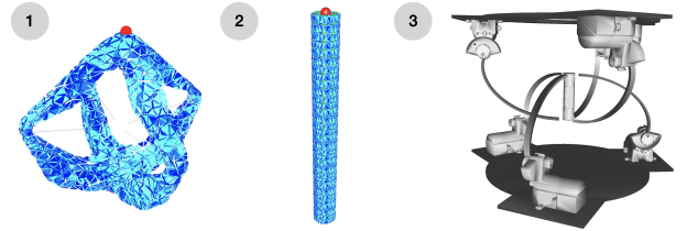
Fig. 3. Representation of the robots used in this work, simulated using SOFA. 1) The Diamond robot. 2) The Stiff-Flop robot. 3) The Liandford robot.
