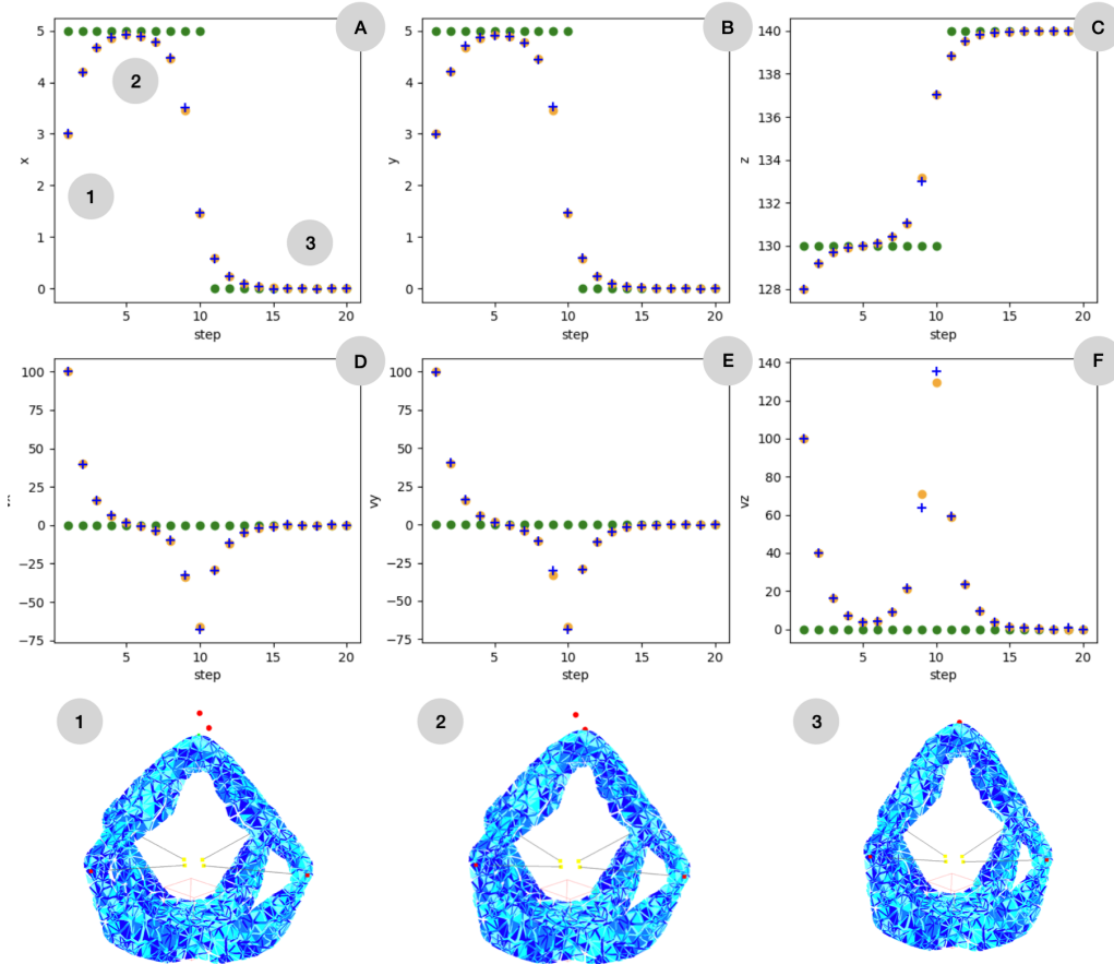
Fig. 4. Results obtained for Diamond robot control. End effector position along x (A), y (B), and z (C) axes. End effector speed along x (D), y (E), and z (F) axes. Green dot: the objective. Blue cross: results obtained by considering the derivative of the non-linear part of the condensed dynamics. Orange dot: results obtained by considering only the linear part. Three robot positions along the trajectory (1, 2, 3) are shown.
