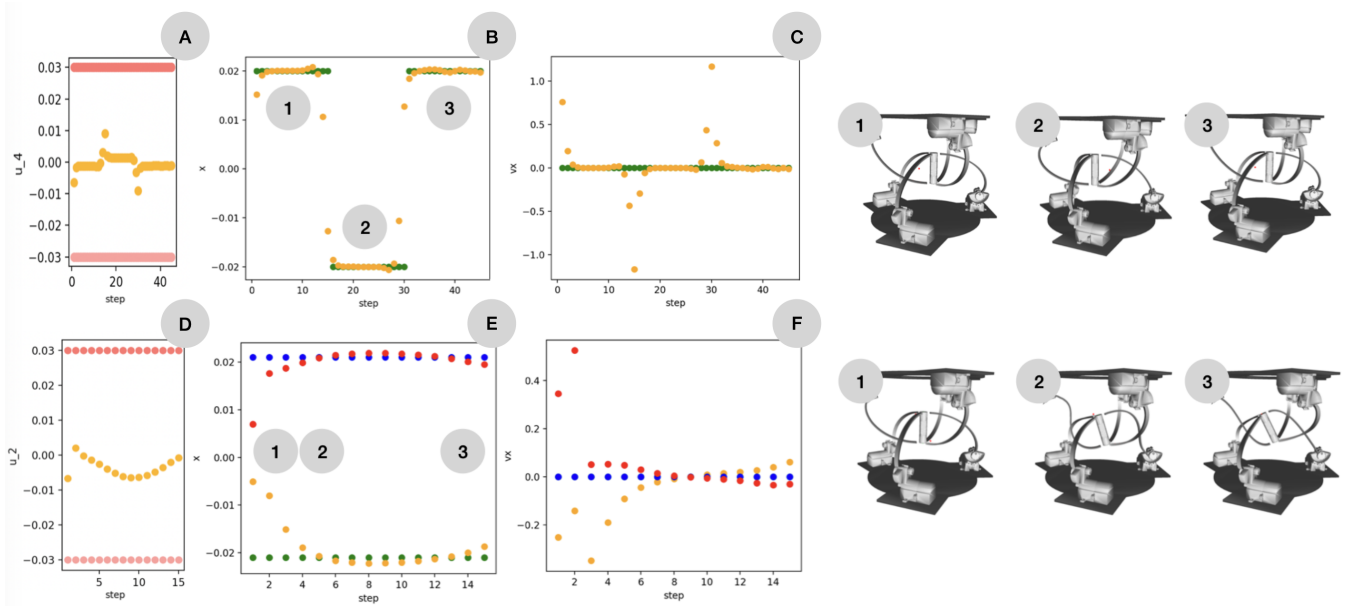
Fig. 7. Results obtained for the Liandford robot control for the second and third cases. First row: actuation (A), position (B), velocity (C), and three configurations of the robot for the pick and place task. Green: the objective. Orange: position and velocity of the effector. Pink: actuation bounds. Second row: actuation (D), position (E), velocity (F), and three configurations of the robot for the orientation task. Green and Blue: the objective. Orange and Red: position and velocity of the effector. Pink: actuation bounds.
