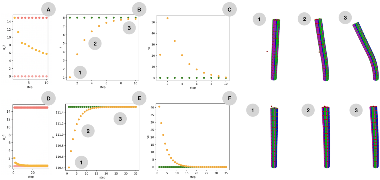
Fig. 5. Results obtained for the Stiff-Flop robot. First row: Effector at the middle of the robot. Second row: Effector at the end of the robot. Example of actuation (A-D); position of the effectors along one axis (B-E); velocity of the effectors along the same axis (C-F); three configurations of the robots (1, 2, 3). Green: the objective. Orange: position and velocity of the effector. Pink: actuation bounds.
