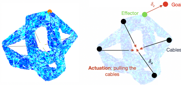
Fig. 1. Example of the Diamond soft robot's actuation and end-effector, that will be developed in Section IV. The effector is a particular point on the robot that we want to control. Its position is modified by applying forces on the actuators.
