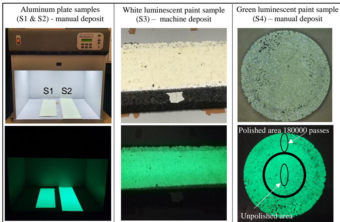
Figure 1 –Left: Aluminium plate samples in the light booth (S1 & S2); Center: White luminescent paint sample S3; Right: Core sample S4 of green luminescent paint artificially ageing with a Wehner & Schulze machine. The ellipses corresponds to the luminance measurement zones.
