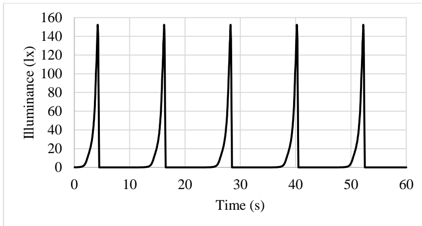
Figure 3. Example of the horizontal illuminance produced on the sample in laboratory with a LED Matrix to simulate a constant traffic at 80 km/h with a vehicle density of 300 veh/h. The figure shows one minute of the signal repeated during six hours in the dark.
