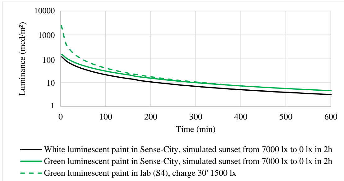
Figure 7: Decay curves in the dark at 2.29° observation angle. Solid lines: in Sense-City after a simulated sunset from 7000 lx to 0 lx in 2 hours; Dotted line: sample S4 of the same green luminescent paint measured in laboratory 30 min of excitation under 1500 lx in a light booth (D65 illuminant + UV)
