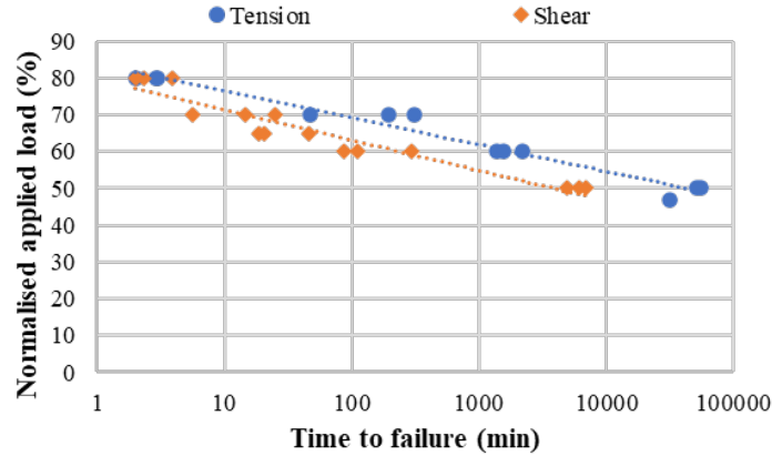
Fig. 6. Normalised applied load as a function of the logarithm of the time to failure
