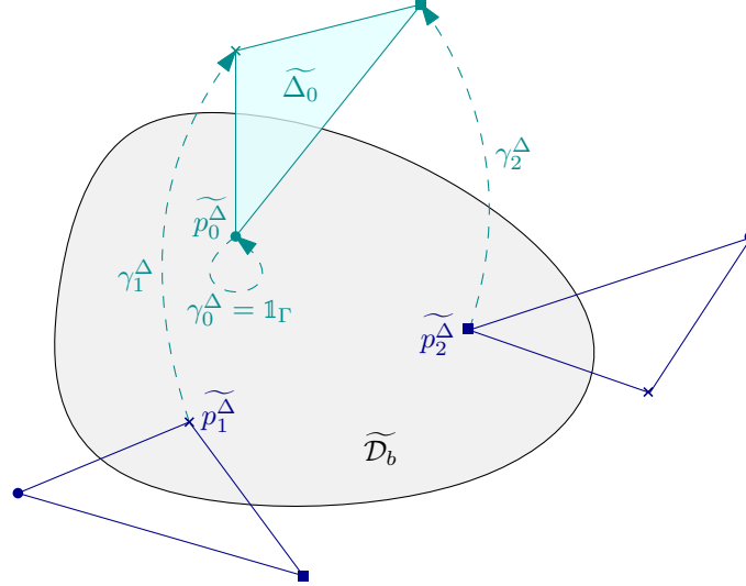
Figure 3: Example of a triangle \Delta having three lifts with one vertex in \mathcal{D}_b^\sim (the hyperbolic triangles are schematically represented with straight edges).
