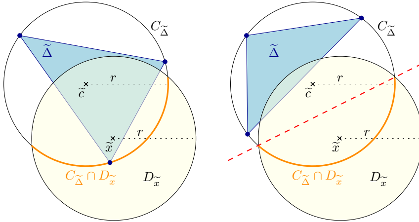
Figure 4: Illustration of the proof of Lemma 2 in Euclidean geometry (for simplicity). The points \tilde{c} and \tilde{x} belong in each other's disk of radius r . Left: If no vertex of \tilde{\Delta} lie on C_{\tilde{\Delta}} \cap D_{\tilde{x}} (bold), then \tilde{x} is separated from \tilde{\Delta} by the dashed geodesic.
