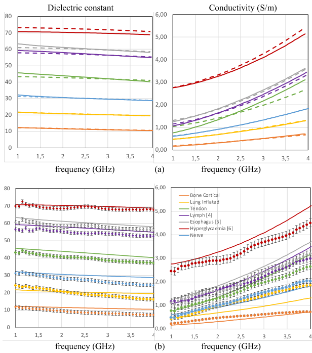
Fig. 2. Comparison between SUPELEC RECIPES mixtures dielectric properties and the reference values provide from literature for seven tissues. (a) prediction (b) measurements
