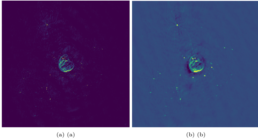
Figure 6: Reconstructed image using algorithm 2 (a) and the CLEAN algorithm (b) on a real radio interferometric observation from the Very Large Array telescope [31].
