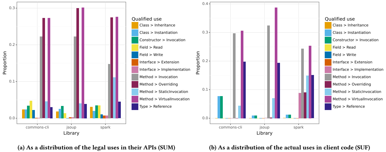
Figure 2: Usage profiles of the three libraries COMMONS-CLI, JSOUP, and SPARK
