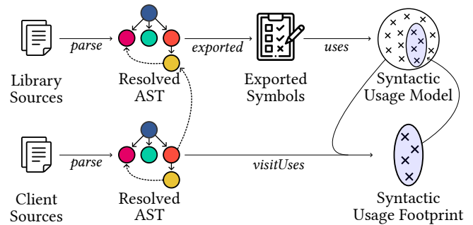
Figure 1: UCov parses and analyses Java code to build SUM and SUF models. Each cross symbol (×) represents one possible use of an API symbol.
