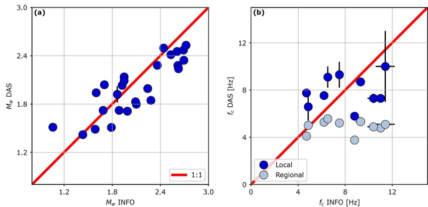
Figure 6. (a) Moment magnitude comparison between estimates from Distributed Acoustic Sensing (DAS) and from Irpinia Near Fault Observatory (INFO) network. Estimates from DAS data follow a 1:1 scaling (red line) when compared with standard seismic station results. (b) Corner frequency comparison between DAS and local network. Without correction for local site effects (gray dots) DAS estimates saturate resulting into an apparent f_c around 5.5 Hz. After the correction for local site effects (blue dots), the two estimates become comparable.
