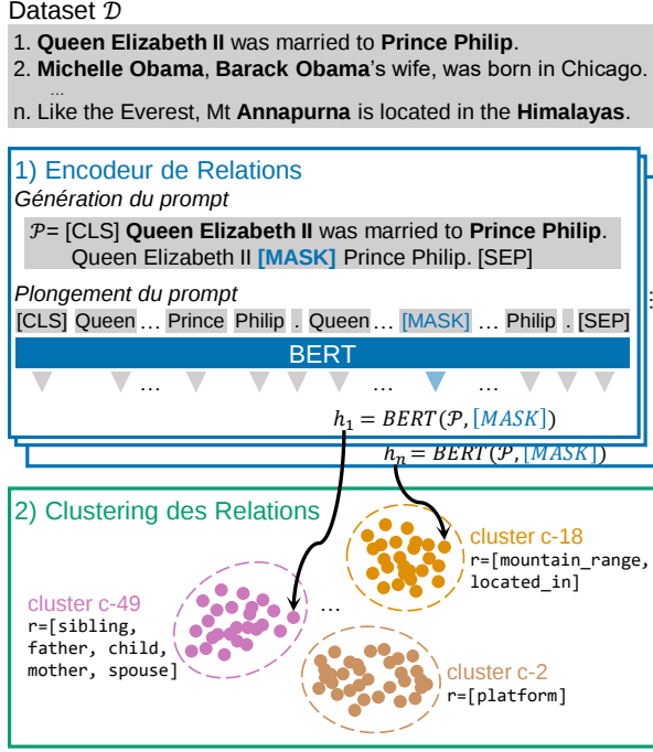
FIGURE 1 – Architecture de PromptORE.
