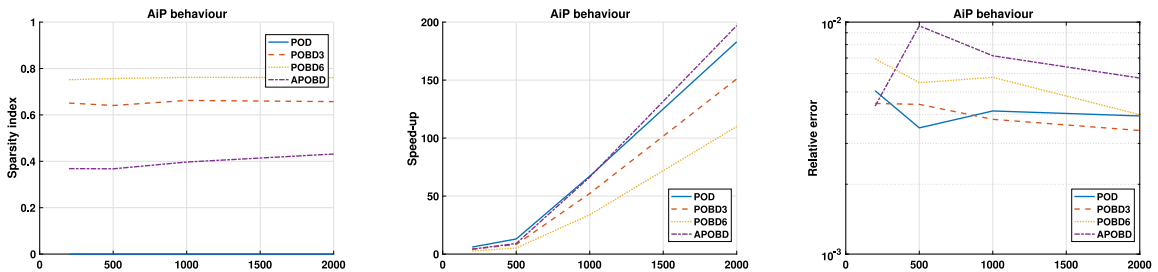
(a) Comparison of the sparsity index for each method in AiP behavior.
