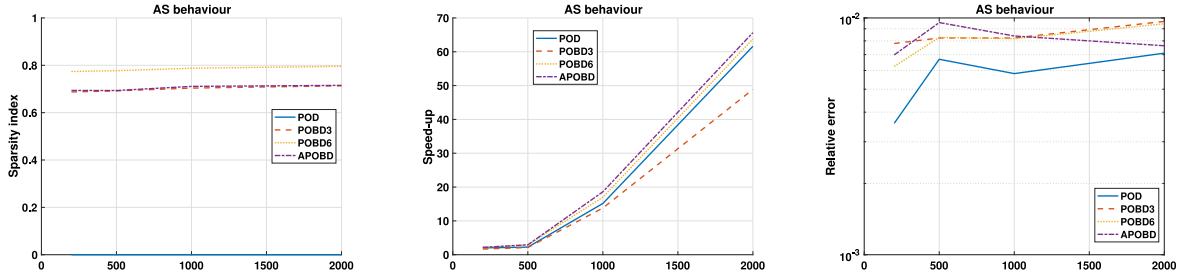
(a) Comparison of the sparsity index for each method in AS behavior. (b) Comparison of the speed-up for each method in AS behavior. (c) Comparison of the relative error for each method in AS behavior.
