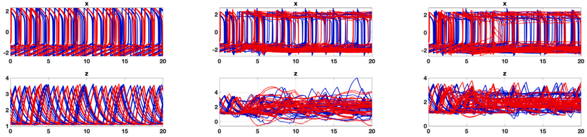
(a) Solution obtained solving system (13) with N = 100 for c_\alpha = -0.5 and c_\beta = 0 . (b) Reduced solution of system (13) with N = 100 for c_\alpha = -0.5 and c_\beta = 0 by means of the POD method. (c) Reduced solution of system (13) with N = 100 for c_\alpha = -0.5 and c_\beta = 0 by means of the POBD method with 3 blocks.
