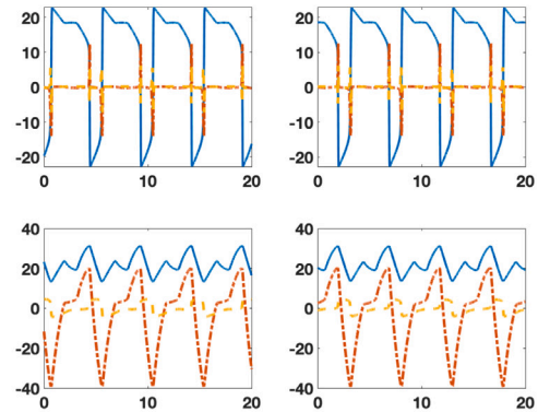
(d) First three basis for each block of the APOBD method for N = 200 cells in AS behavior.
