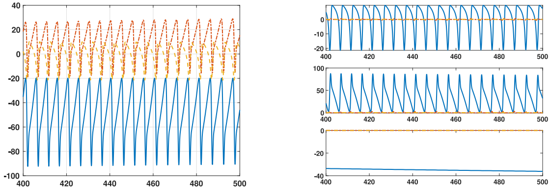
(a) First basis for the POD method for N = 100 cells in sustained oscillation behavior. (b) First basis for each block of the APOBD method for N = 100 cells in sustained oscillation behavior.
