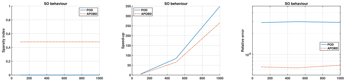
(a) Comparison of the sparsity index for each method in SO behavior. (b) Comparison of the speed-up for each method in SO behavior. (c) Comparison of the relative error for each method in SO behavior.
