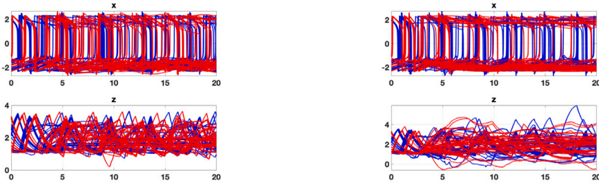
(d) Reduced solution of system (13) with N = 100 for c_\alpha = -0.5 and c_\beta = 0 by means of the POBD method with 6 blocks. (e) Reduced solution of system (13) with N = 100 for c_\alpha = -0.5 and c_\beta = 0 by means of the APOBD method.
