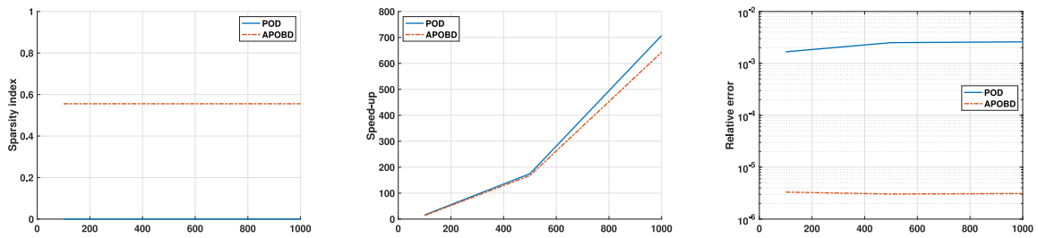
(a) Comparison of the sparsity index for each method in FHB behavior. (b) Comparison of the speed-up for each method in FHB behavior. (c) Comparison of the relative error for each method in FHB behavior.
