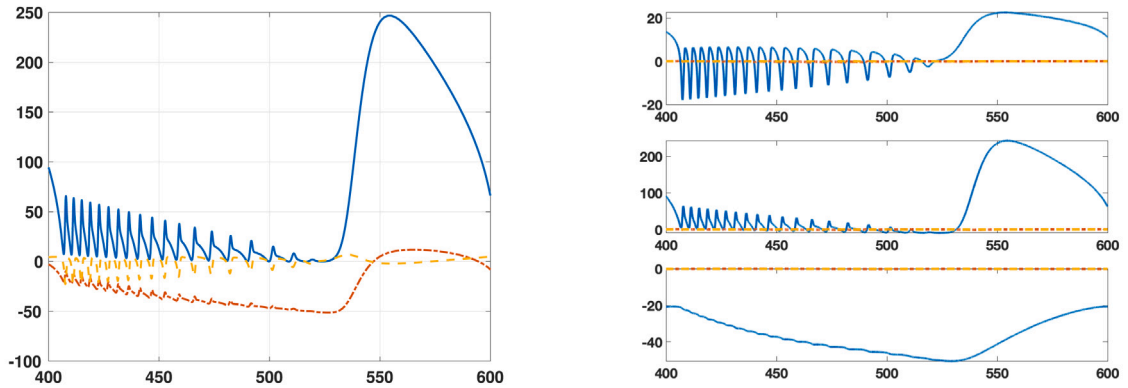
(a) First basis for the POD method for N = 100 cells in PB behavior. (b) First basis for each block of the APOBD method for N = 100 cells in PB behavior.
