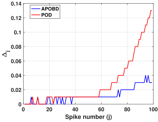
(a) Comparison of the error estimators for sustained oscillation behavior of system (14) with N = 100 cells.
