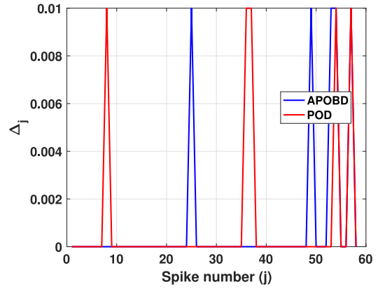
(b) Comparison of the errors for PB behavior of system (14) with N = 100 cells.
