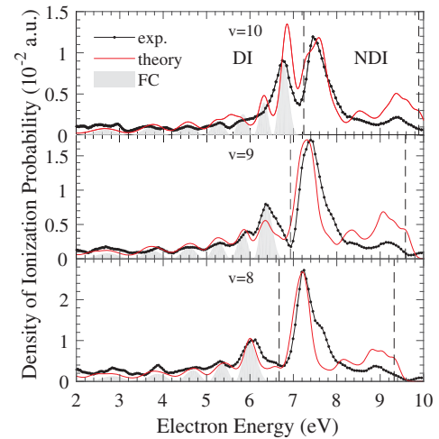
FIG. 4. Experimental and theoretical photoelectron spectra for B^1\Sigma_u^+ ( v = 8-10 ). The gray shaded areas depict the FC overlap between the B(v) state with the H_2^+(2p\sigma_u^2\Sigma_u^+) continuum.
