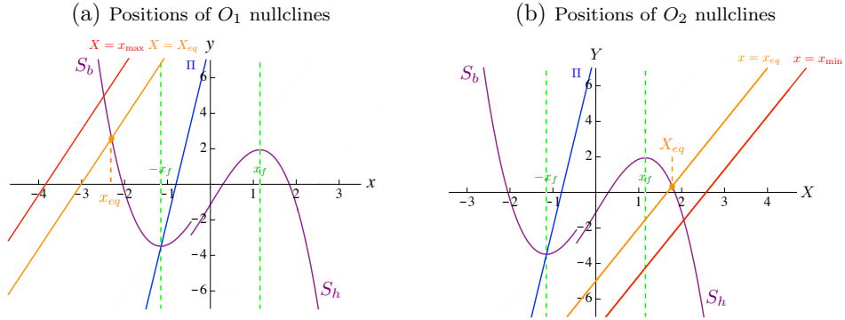
Figure C.18: Projections of the nullclines of oscillators O_1 (panel (a)) and O_2 (panel (b)) with parameter values given by 11 and c = -0.7 < c^d . We represent in the same plane the two planes z = z_b for x < x_{on} and z = z_h for x > x_{on} . In purple, the special curves of the critical manifold S_b and S_h given in eq. (9); in blue, the plane \Pi (uncoupled case); in red, y -nullcline for X = x_{\max} (panel (a)) and the Y -nullcline for x = x_{\min} (panel (b)); in orange, the y and Y -nullclines for x = x_{eq} and X = X_{eq} corresponding to the stable quasi-equilibrium point of the coupled system. We also represent in green the lines x = -x_f and x = x_f .
