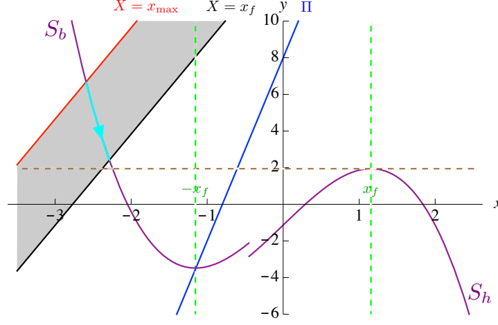
Figure C.19: Projections of the nullclines of oscillator O_1 with parameter values given by 11, c = -0.502 and X decreasing from x_{\max} to x_f . We represent in the same plane the two planes z = z_b for x < x_{on} and z = z_h for x > x_{on} . In purple, the special curves of the critical manifold S_b and S_h given in eq. (9); in blue, plane \Pi corresponding to the uncoupled case; the grey area materialize the locus of plane \Pi_c for X between x_{\max} (red line) and X = x_f (black line). Considering X decreasing between these values, O_1 current point stays close to the stable singular point, which follows the cyan trajectory. The dashed green lines materialize the x -component of the folds x = -x_f and x = x_f and in brown the fast fibers corresponding to the upper fold \mathcal{F}^+ . In the case of relaxation loss of O_1 , its singular point remains above (i.e. has a greater y -component than) the upper fold: the intersection of the black line with the purple curve is above the dashed brown line.
