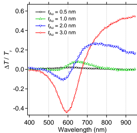
Fig. 3: Difference in transverse and longitudinal transmittances \Delta T = T_y - T_x divided by the transverse transmittance T_y with increasing effective thicknesses from t_{\text{Au}} = 0.5 nm to t_{\text{Au}} = 3.0 nm.
