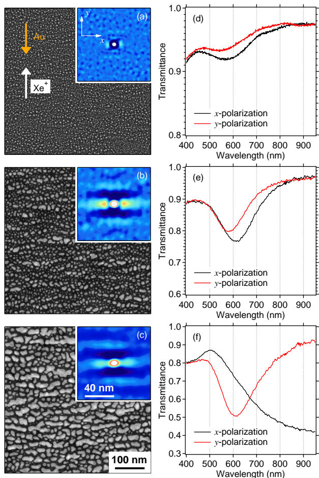
Fig. 2: Plane-view HAADF-STEM images of rippled \text{Al}_2\text{O}_3 thin films after glancing-angle Au deposition. The effective Au thicknesses are (a) t_{\text{Au}} = 0.5 nm, (b) t_{\text{Au}} = 1.0 nm, and (c) t_{\text{Au}} = 3.0 nm. The directions of the \text{Xe}^+ beam and Au flux are indicated by the arrows, and the autocorrelation functions of the images are shown in the insets. (d-f) Corresponding transmission measurements at normal incidence with the polarization of the incoming light being oriented parallel ( x -polarization) and perpendicular ( y -polarization) to the ripples.
