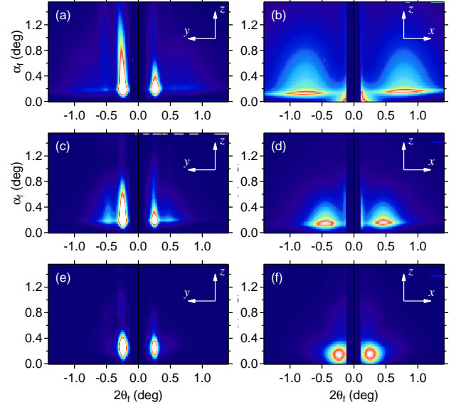
Fig. 4: Experimental GISAXS patterns of rippled \text{Al}_2\text{O}_3 thin films after glancing-angle Au deposition. (a) t_{\text{Au}} = 0.5 nm and x-rays along the x -direction, (b) t_{\text{Au}} = 0.5 nm and x-rays along the y -direction, (c) t_{\text{Au}} = 1.0 nm and x-rays along the x -direction, (d) t_{\text{Au}} = 1.0 nm and x-rays along the y -direction, (e) t_{\text{Au}} = 3.0 nm and x-rays along the x -direction, (f) t_{\text{Au}} = 3.0 nm and x-rays along the y -direction.
