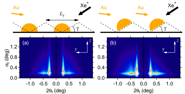
Fig. 5: Simulated GISAXS patterns ( t_{\text{Au}} = 1.0 nm and x-rays along the x -direction) by assuming that the Au nanoparticles are (a) in the ripple valleys and (b) tilted from the surface normal by a tilt angle of \gamma .
