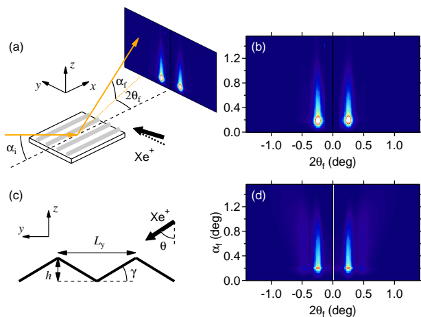
Fig. 1: (a) Schematic drawing of the GISAXS geometry. (b) Experimental GISAXS pattern of a rippled \text{Al}_2\text{O}_3 thin film with the incident x-ray beam along the x -direction. (c) Schematic drawing of the model surface profile. (d) Simulated GISAXS pattern with the parameters obtained from the fit of the experimental map.
