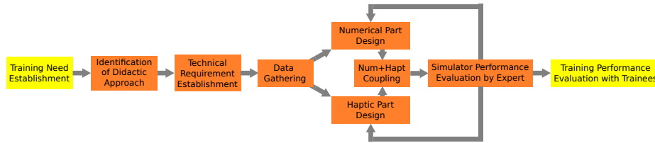
Fig. 2. Haptic Training Simulator Design Process.
