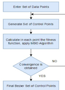
Figure 1: Bezier Curve Fitting using MBO algorithm
