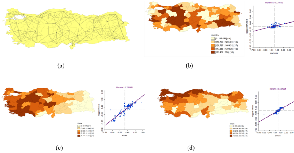
Figure 1: (a)Linkage map indicating the neighborhood relationship, (b)The global moran i graph and the cluster map for AQI in 2014, (c)The global moran i graph and the cluster map for the number of cars per person in 2014, (d)The global moran i graph and the cluster map for the annual average humidity
