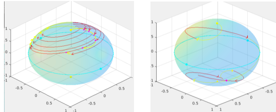
Figure 1: Red color curves are for control u = +1 , yellow color curves are for control u = -1 , the cyan curve is singular locus. In left figure: Normal, bang; bang-bang; bang-bang-bang; bang-bang-bang-bang; bang-bang-bang-bang-bang optimal trajectories. In the right side figure : Abnormal, bang-bang-bang-bang-bang-bang optimal trajectory.
