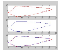
Figure 2: The result of Bezier Curve Fitting using MBO algorithm
