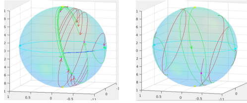
Figure 2 Red color curves are for control u = +1 , green color curves are for control u = -1 , the cyan curve is singular locus, blue curve is singular optimal trajectory, and magenta color points are cut locus points. Left figure : Normal, bang; bang-bang; bang-singular-bang; bang-bang-bang optimal trajectories. Right side figure: Abnormal bang-bang...bang-bang optimal trajectory, magenta color point is cut locus point.
