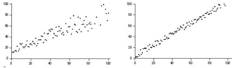
Figure 1: The first graph shows heteroscedasticity and the other graph shows homoscedasticity
