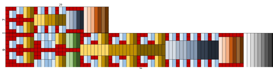
Figure 3: The patterns of n -color palindrome compositions of 7 and 9 such that the middle part is n -color
