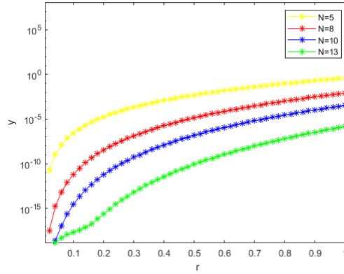
Figure 2: Comparising approximate solution for N=5,8,10 and 13 of Example 2
