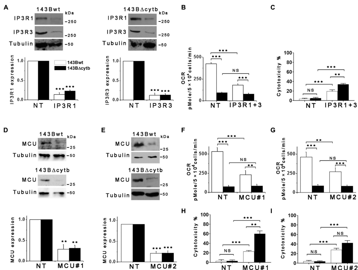
Fig. 2. Simultaneous knockdown of types 1 and 3 \text{InsP}_3\text{R} or mitochondrial \text{Ca}^{2+} uptake induces cell death in OXPHOS-defective 143B \Delta\text{cytb} cells.
