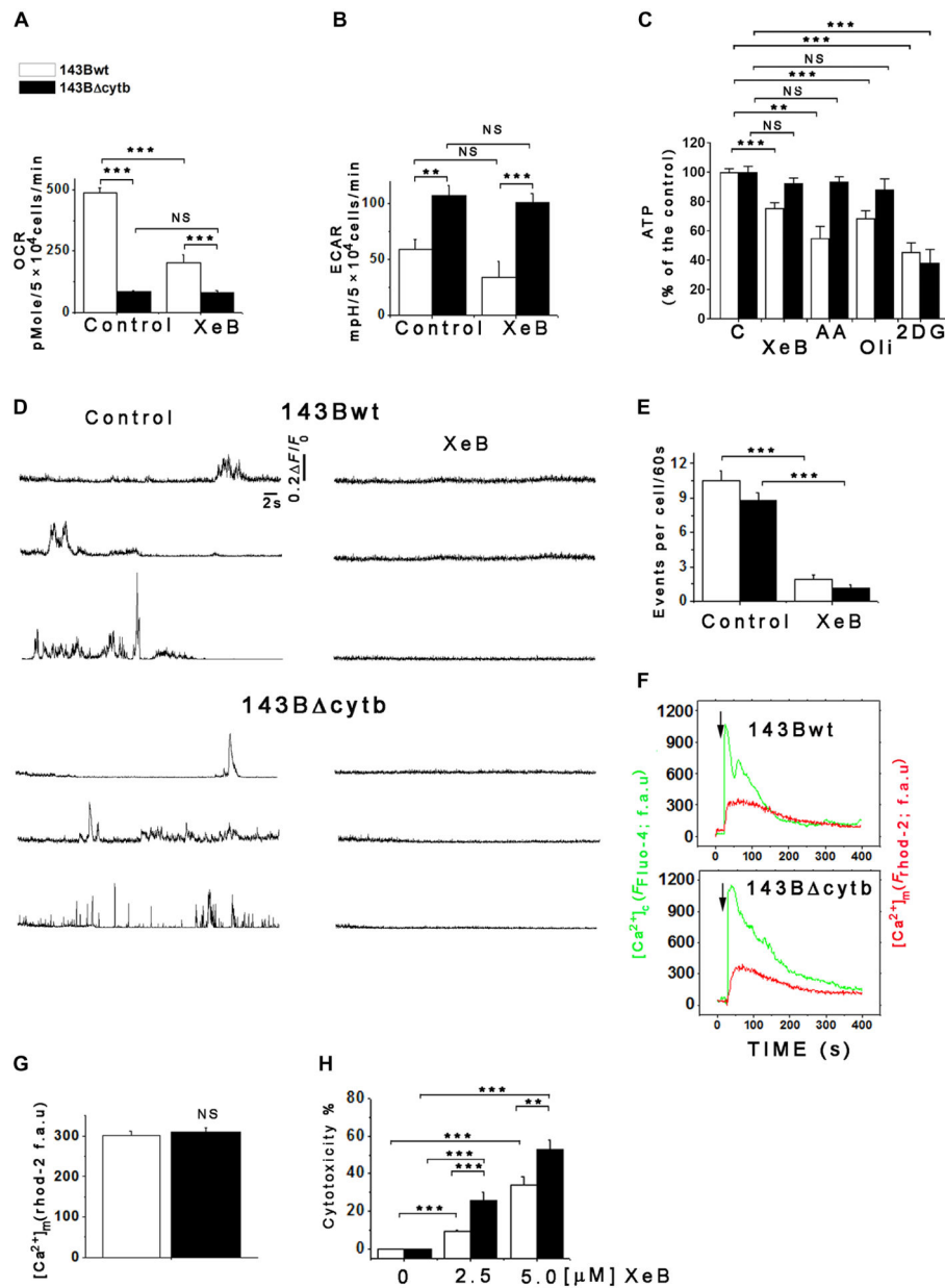
Fig. 1. OXPHOS-defective 143BΔcytb cells rely on constitutive InsP 3 R-mediated Ca 2+ signals. (A) Basal oxygen consumption rate (OCR) of cells incubated with 5 μM XeB for 4 hours. (B) Extracellular acidification rate (ECAR) of cells incubated with 5 μM XeB for 4 hours. Data in (A) and (B) represent means ± SEM of three independent experiments with 10 replicates each. ** P < 0.01 and *** P < 0.001 compared to respective control. NS, not significant. (C) Cells were incubated with 5 μM XeB, 1 μM antimycin A (AA) or 1 μM oligomycin (Oli), 2-deoxyglucose (2DG; 20 mM), or vehicle control (C) for 4 hours, and intracellular ATP levels were determined. Means ± SEM of three independent experiments performed in triplicate. *** P < 0.001 compared to control. (D) Representative recordings of Ca 2+ release events in unstimulated cells treated or not with 5 μM XeB for 30 min. (E) Quantification of Ca 2+ release events. Means ± SEM of three independent experiments.
