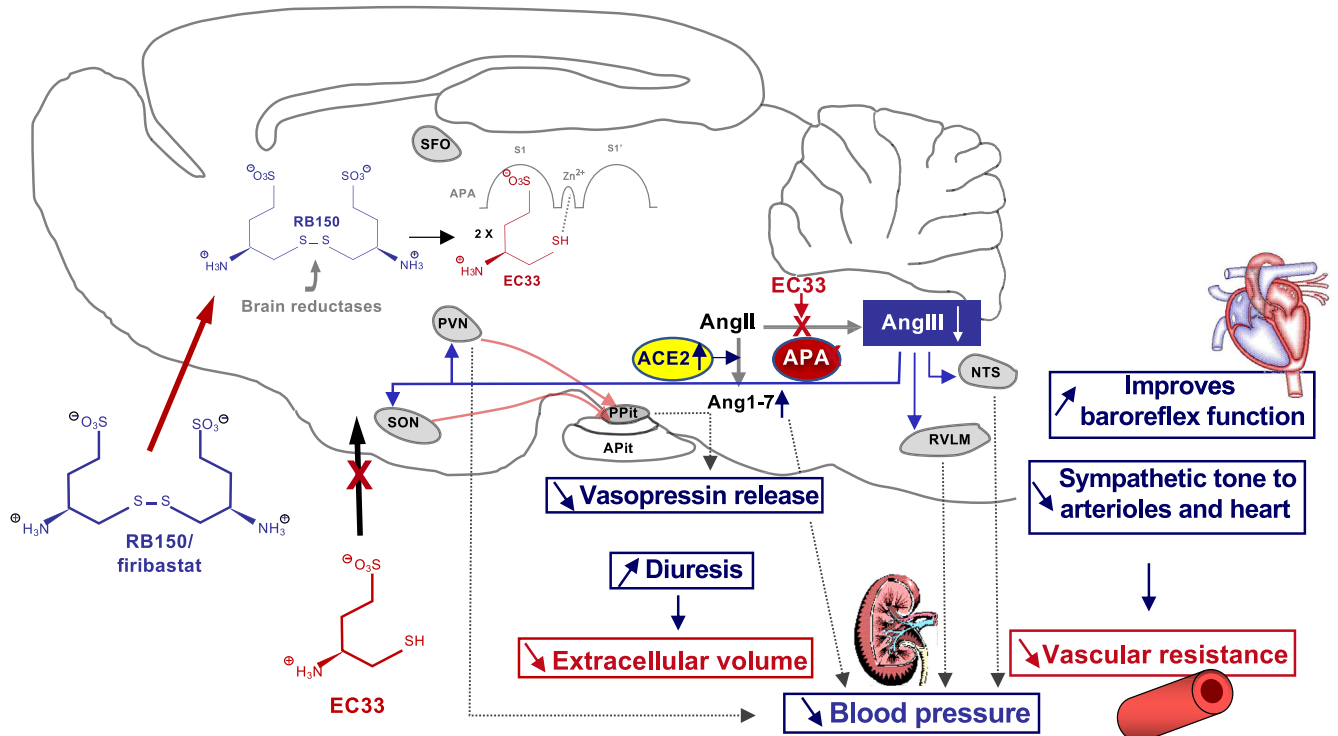
Figure 1. (A) Pharmacologic and structural properties of the aminopeptidase A (APA) inhibitors EC33 and NI929, and their prodrugs, RB150/firibastat, NI956, and QGC606. 16,25,26 The S1 subsite is visualized in the 3-dimensional (3D) model of human APA after molecular docking of EC33 (orange). 24 Molecular docking of NI929 (blue) in the 3D model of human APA is also shown. 25 (B) Mode of action of the APA inhibitor prodrug, RB150/firibastat, on the control of blood pressure in hypertensive rats (Modified from Marc et al 27 with permission from Hypertension and
