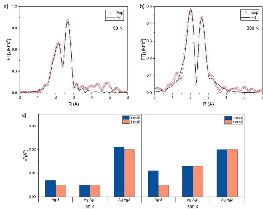
Figure 6. Ag K-edge FT-EXAFS spectrum of \text{Ag}_{44}(\text{SR})_{30} with four-shell fitting at a) 90 K and b) 300K. c) The comparison of Debye-Waller factors obtained by two fitting methods. The Debye-Waller factors for two Ag-S shells were correlated for four-shell fitting method, so they have the same value and only one bar was shown in the figure (Left panel: 90 K; right panel: 300K).
