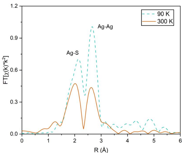
Figure 1. Ag K-edge FT-EXAFS spectra of \text{Ag}_{44}(\text{SR})_{30} at 90 K and 300 K.
