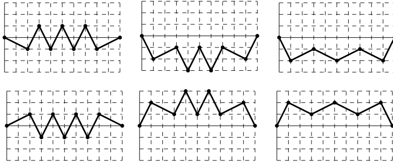
Figure 4: The six grand zigzag knight's paths of size 10 having exactly the starting and the ending point on the x -axis.
