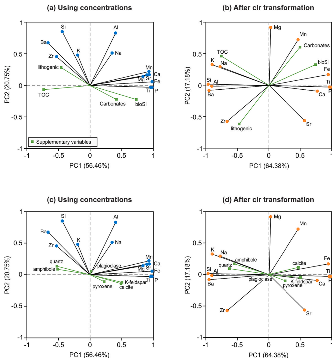
Fig. 9. PCA of the geochemical composition of fjord sediment core PC29A, with sediment composition (a–b) and mineralogy (c–d) plotted as supplementary variables. Data from Bertrand et al. (2014).
