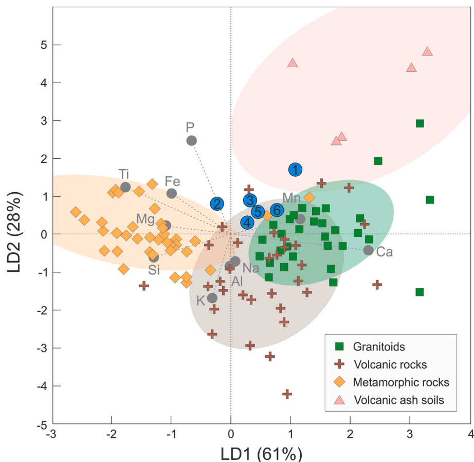
Fig. 12. Linear discriminant biplot of sediment sources (105 bedrock samples and 5 soil samples) from Chilean Patagonia (Liu et al., 2020). The ellipses represent the confidence intervals (1 sigma). The blue circles correspond to river sediment samples draining different watersheds. The plot shows that sample 1 has a distinct provenance and is particularly enriched in volcanic ash soil material. Figure modified from Liu et al. (2020).
