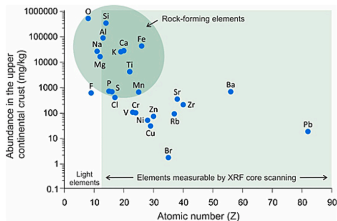
Fig. 1. Abundance of elements in the Earth's upper continental crust (from Rudnick and Gao, 2014) plotted against their atomic number. For elements with Z > 12 , only those detectable by XRF core scanners are shown. Note that Na, Mg and O are important rock-forming elements but that they are not measurable by XRF-CS. Figure inspired from Rothwell and Croudace (2015).
