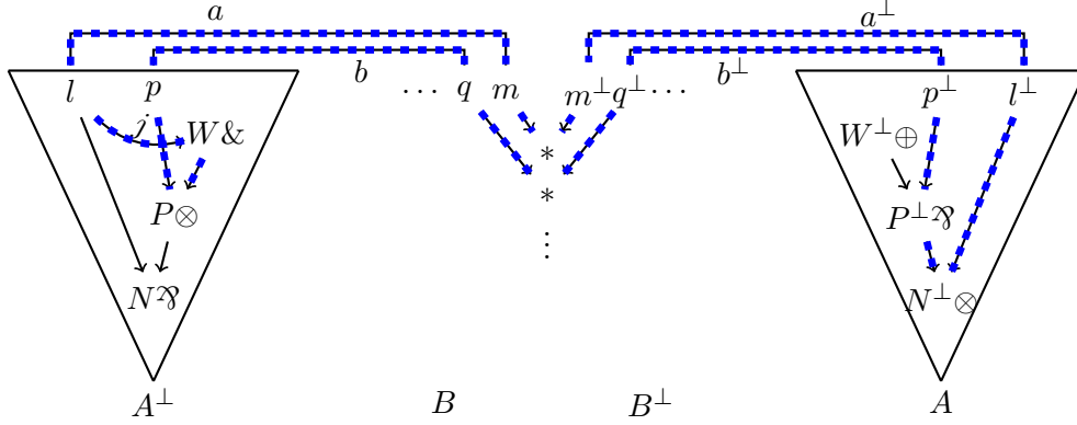
Figure 11: Switching cycle containing W if P is a \otimes -vertex in the proof of Lemma 8.18
