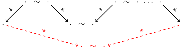
Figure 16: Diagram of Church-Rosser modulo \sim (Definition A.1), with hypotheses in solid black and conclusions in dashed red
