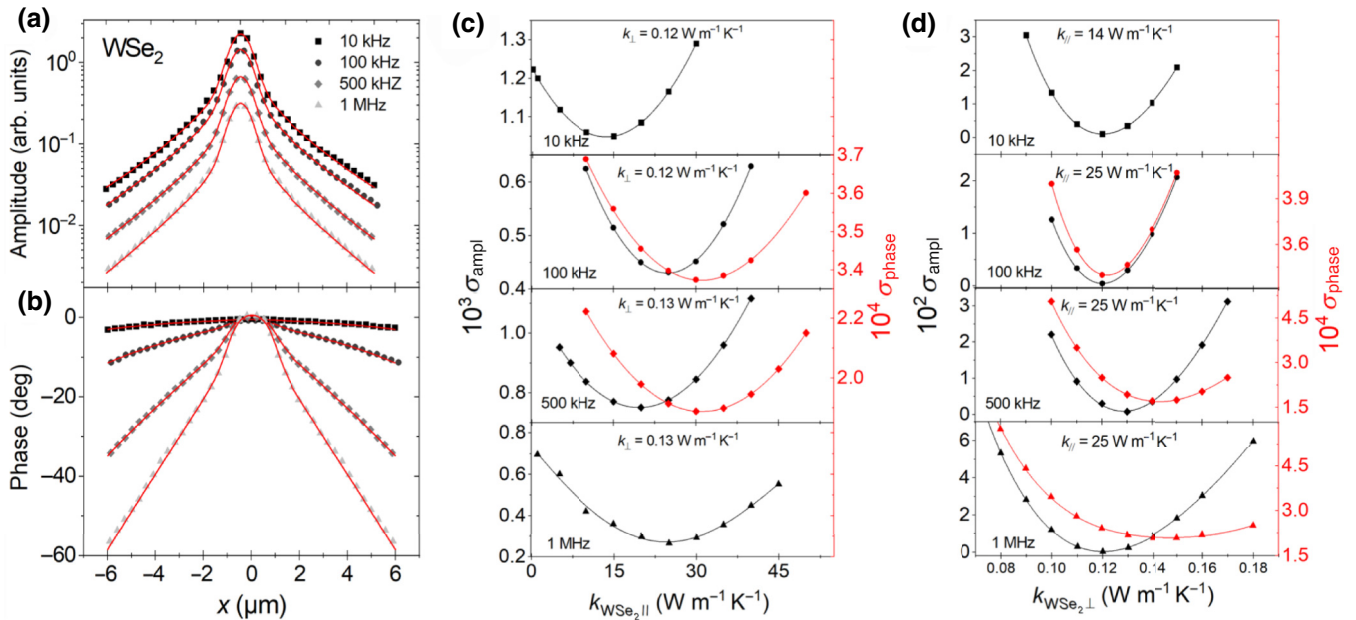
FIG. 6. (a) MTR amplitude and (b) phase data (points) and the corresponding best fits (solid lines) measured on WSe 2 of sample S1 at four modulation frequencies (10 kHz, 100 kHz, 500 kHz, and 1 MHz). Experimental data and best-fit curves are vertically translated for the sake of clarity. (c) Calculated variance of the amplitude, \sigma_{\text{ampl}} (black points—left axis), and phase signal, \sigma_{\text{phase}} (red points—right axis), as a function of k_{\text{WSe}_2\parallel} while fixing k_{\text{WSe}_2\perp} at the value indicated in each plot for data acquired at 10 kHz, 100 kHz, 500 kHz, and 1 MHz (from the top to the bottom). Solid black and red lines are the best polynomial fits of the data. (d) Calculated variance of the amplitude, \sigma_{\text{ampl}} (black points—left axis), and phase signal, \sigma_{\text{phase}} (red points—right axis), as a function of k_{\text{WSe}_2\perp} while fixing k_{\text{WSe}_2\parallel} at the value indicated in each plot for data acquired at 10 kHz, 100 kHz, 500 kHz, and 1 MHz (from the top to the bottom). Solid black and red lines are the best polynomial fits of the data.
