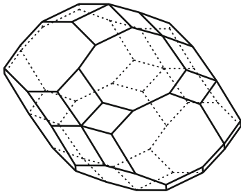
(A) A generic 2nd higher 5-permutahedron.
