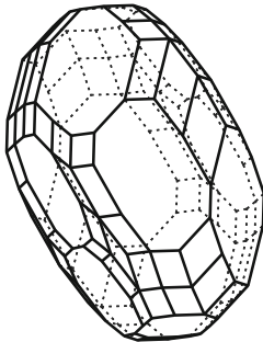
(C) A generic 3rd higher 6-permutahedron.
