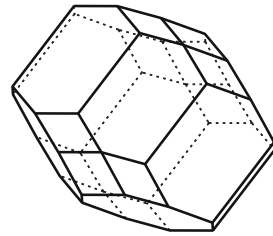
(B) A degenerate 2nd higher 5-permutahedron.
