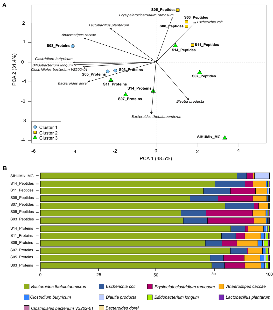
Fig. 5 Comparisons of community composition for SIHUMix at the species level. The upper panel shows PCA clustering of the results (A). Different approaches and tools used for taxonomic annotation (MG - mOTU2, Peptides - UniPept, and Proteins - ProPhane) are indicated in the label. Clusters ( k = 3 ) were calculated using manhattan distance and are represented by blue, yellow, and green. Features not annotated at species level were considered unclassified and discarded for PCA calculation. Unclassified features accounted for 24.2% and 69.9% of data for peptide and protein subgroup levels. Variables driving differences between samples are represented by black arrows. The lower panel details taxonomic profiles of each sample as bar plots (B). Source data is provided as a Source Data file.
