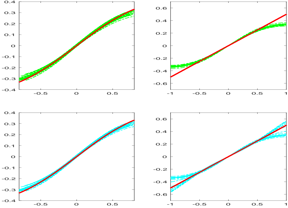
FIGURE 2. Example 2, T = 2000 . 20 estimated b (left) and \phi (right), all selected by penalization (top green) or as oracles (bottom cyan). The true functions are in bold red.
