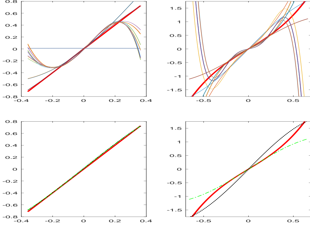
FIGURE 4. Example 5, T = 200 . First line: the 6 \times 3 proposals for b (left) and the 3 \times 6 proposals for \phi (right). Second line: \hat{b}_2 (left) and \hat{\phi}_1 (right) selected by penalization (green) or oracle (dotted black). In all cases, the true is in bold red.
