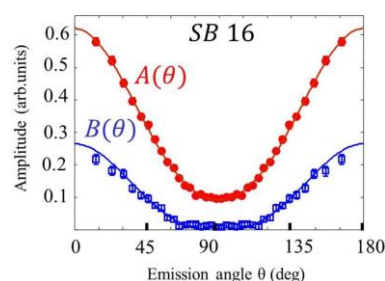
Figure 1 A(\theta) and B(\theta) for SB16 in XUV+IR PI of Ar. reduced set of coefficients, which allows for generating e.g. the A(\theta) , B(\theta) and C(\theta) functions, will be presented. First MFPADs, obtained taking advantage of dissociative PI, will also be reported for PI of NO and compared with MCSCI calculations.
