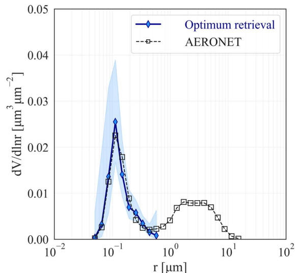
Figure 8. Evaluation of the retrieved volume size distribution (blue line) of the anthropogenic component, with the AERONET volume size distribution (black line with squares), for the case study from the Antikythera EARLINET station on 25 May 2020.
