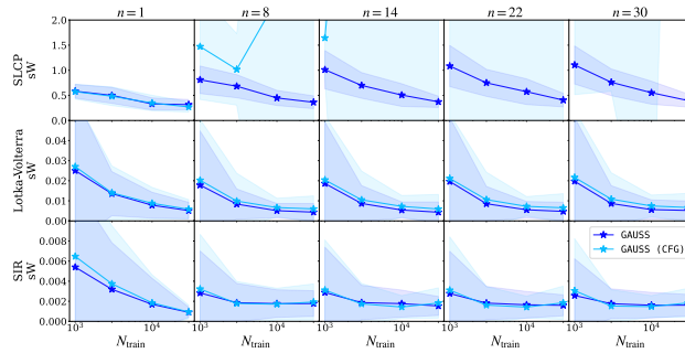
(a) Sliced Wasserstein (sW).
