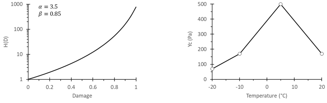
13 14 Fig. 9. (Left) evolution of the softening function H(D) with damage for \alpha = 3.5 and \beta = 0.85 , (Right) evolution 15 of Y_c with temperature 16
