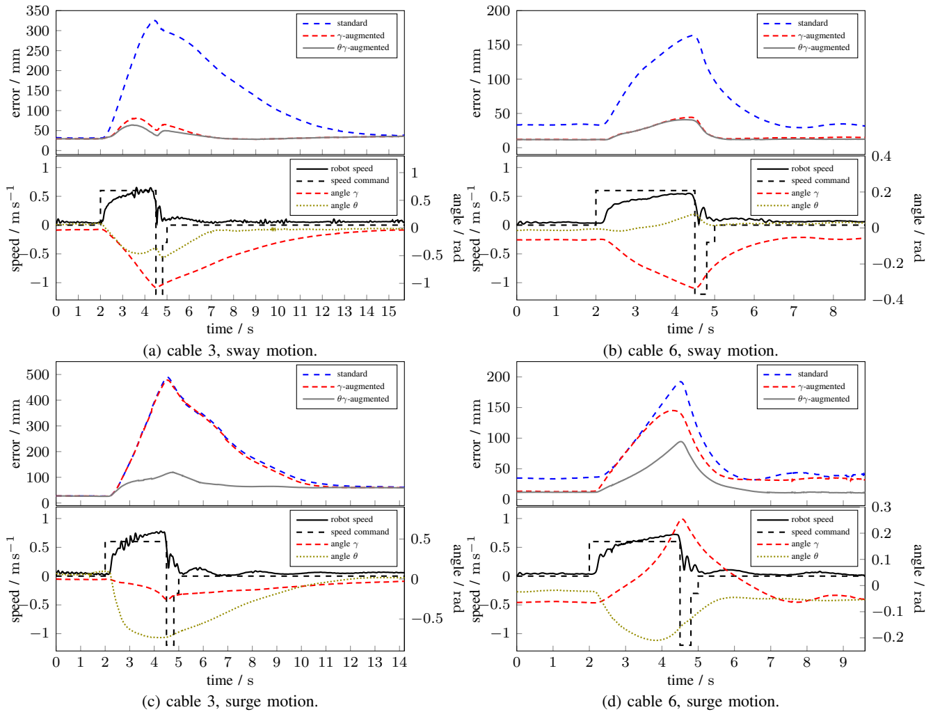
Fig. 8: Model residuals, robot speed and \theta , \gamma angles over time. Speed command of 0.6 \text{ m s}^{-1} and 2 m distance.
